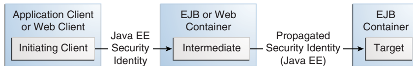
Figure 49–1 Security Identity Propagation
