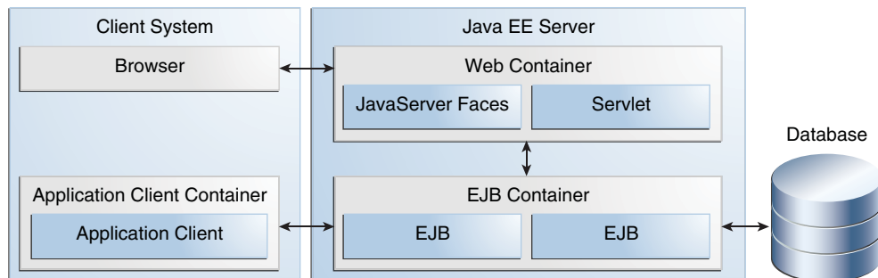
Figure 1–6 Java EE Containers
