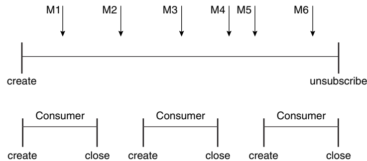
Figure 45–7 Consumers on a Durable Subscription
