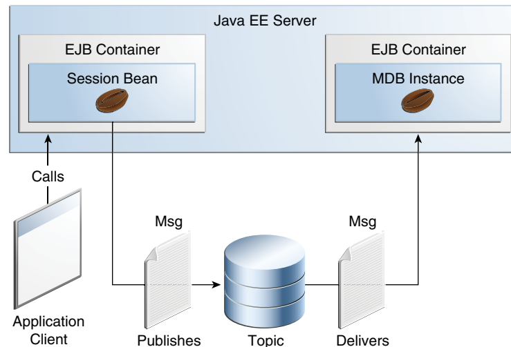
Figure 46-4 An Enterprise Bean Application: Client to Session Bean to Message-Driven Bean
