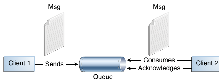
Figure 45–3 Point-to-Point Messaging
