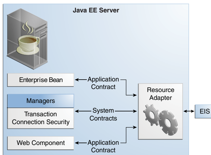
Figure 52-1 Resource Adapters
