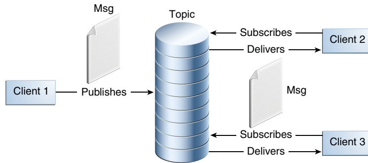
Figure 45-4 Publish/Subscribe Messaging
