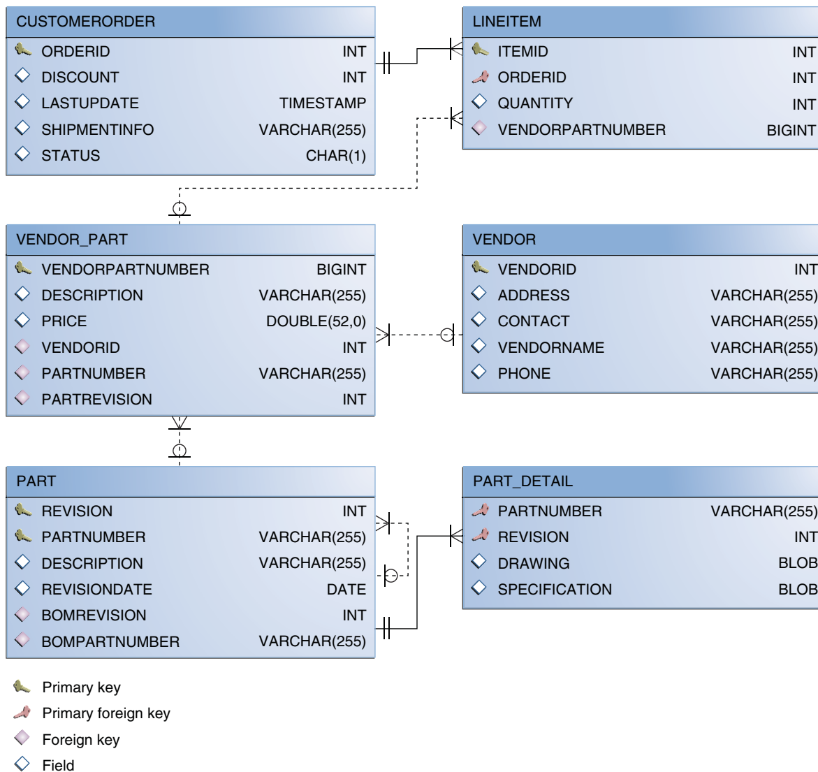
Figure 38-1 Database Schema for the order Application
