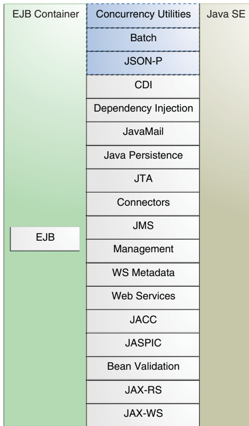
Figure 1–8 Java EE APIs in the EJB Container
