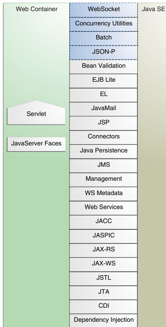
Figure 1–7 Java EE APIs in the Web Container
