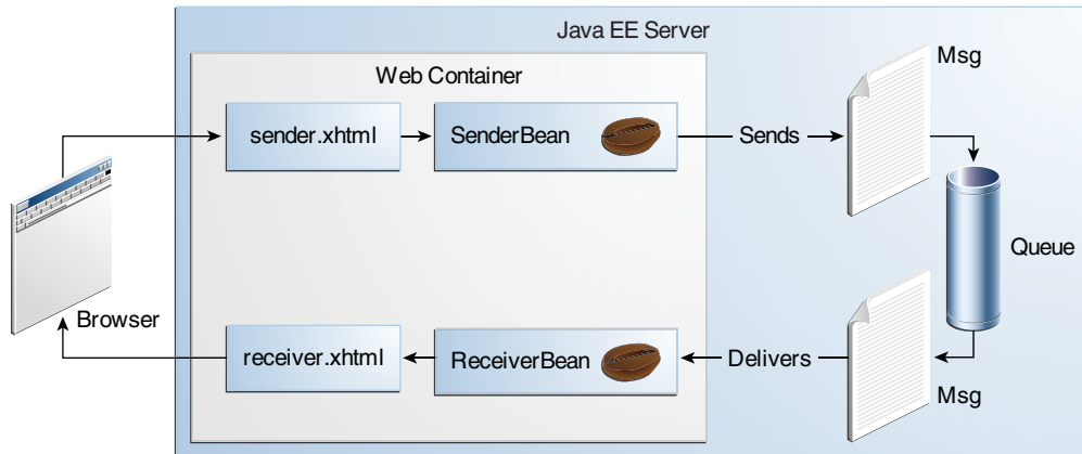
Figure 46–2 The websimplemessage Application
