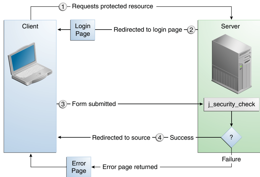
Figure 48–2 Form-Based Authentication
