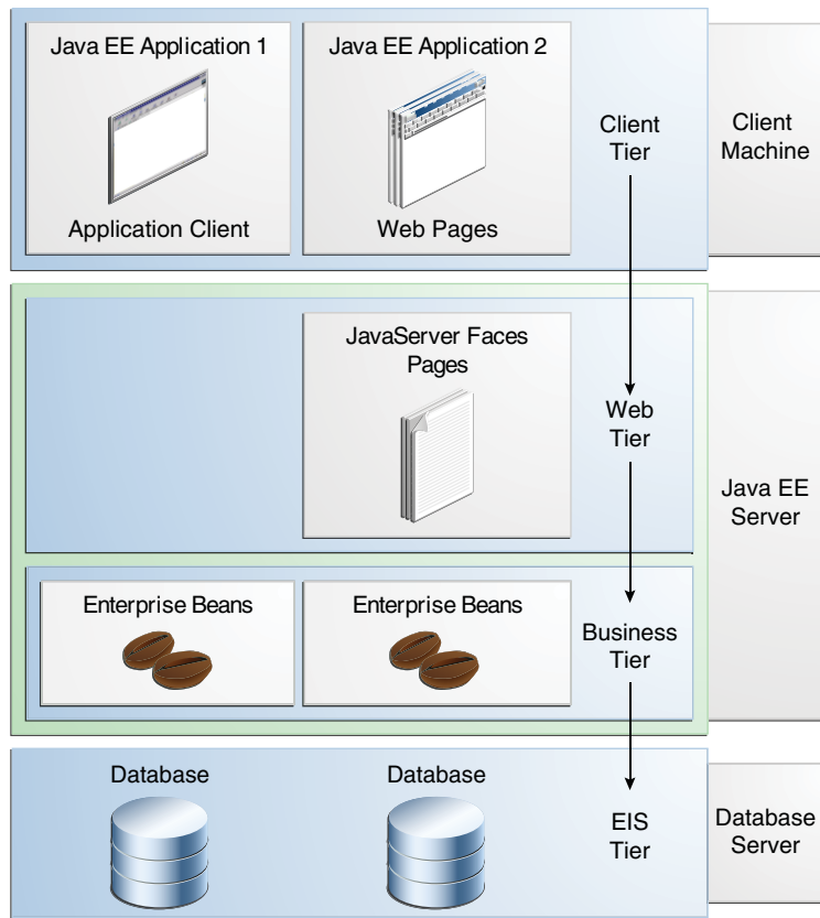
Figure 1-1 Multitiered Applications
